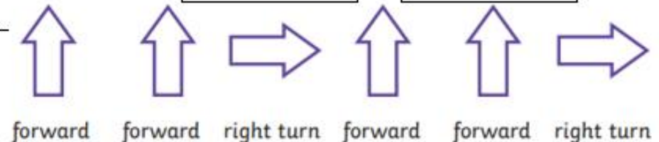
Algorithm
